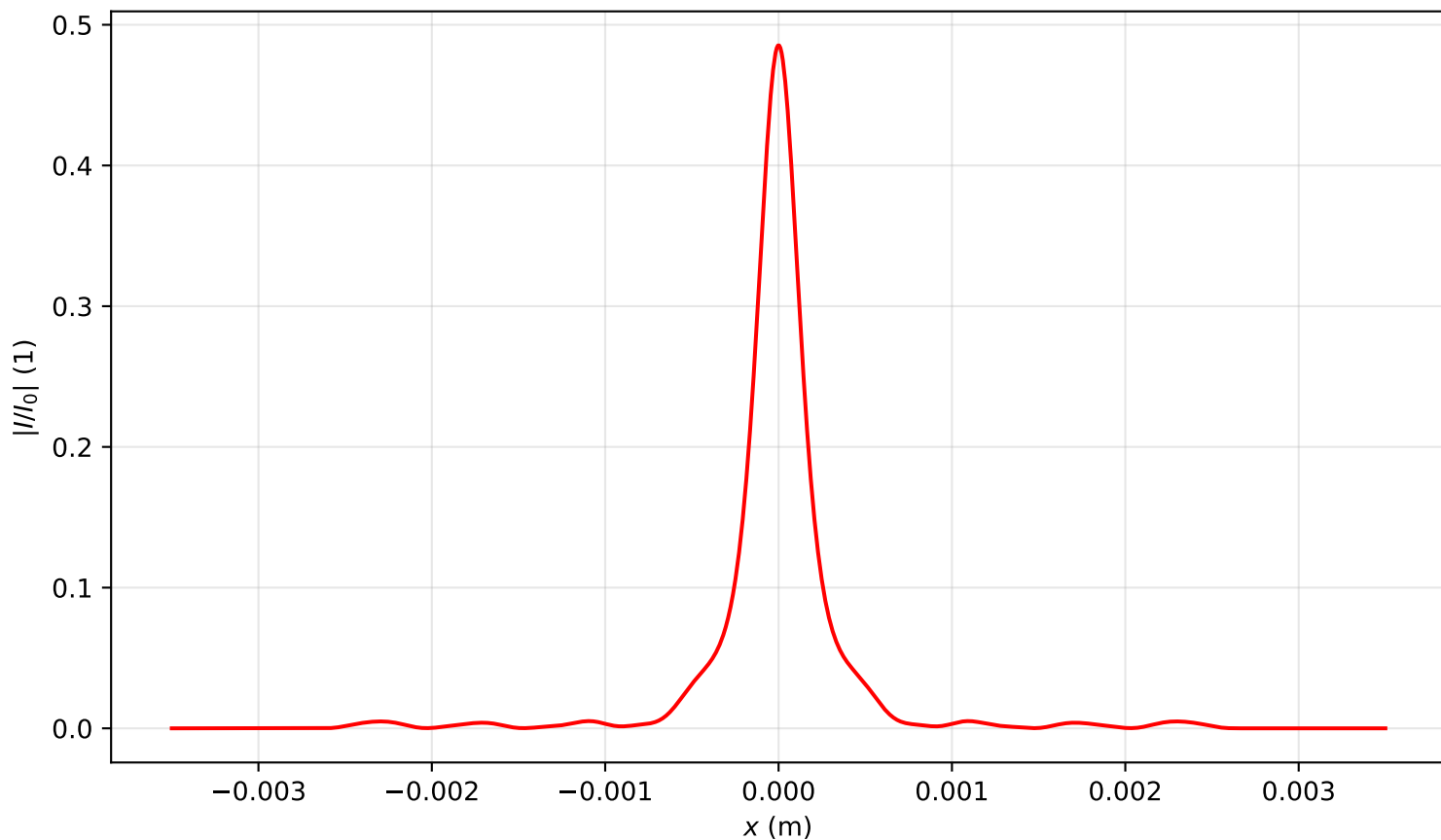
Intensity profile I(x, y = 0, z = 3.821)/I_0 , P_{in}=7.0P_{cr} , artificial time
